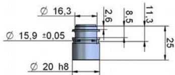
Detail drawing standard flange
