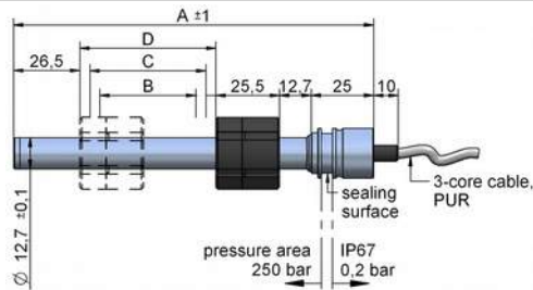
Detail drawing threaded flange
