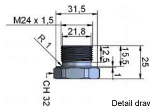
Detail drawing threaded flange
