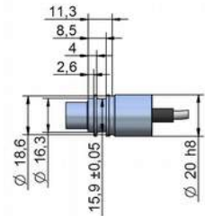
Detail drawing standard flange
